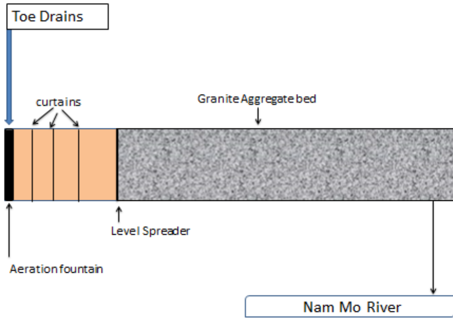
Figure 1 Design of the passive treatment systems
